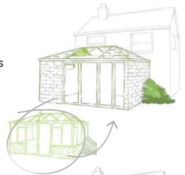
Transformations
